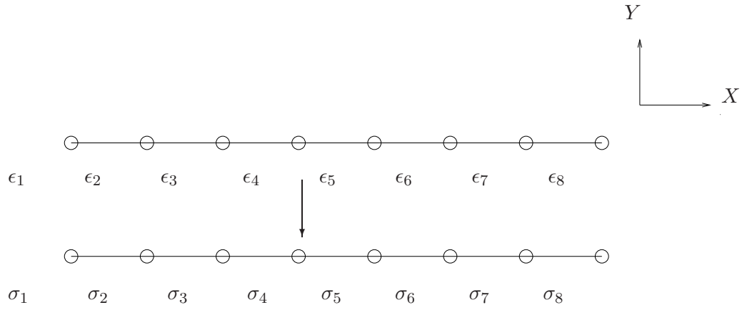
Figure 6.2: Schematic for the 1D local sums algorithm for N = 8 case. Here \epsilon_k denotes the value of a scalar quantity at the k^{th} grid point, while \sigma_k denotes its prefix sum (see Eqs. 6.9 and 6.10). The former can be overwritten by the latter using Eqs. 6.9 and 6.10.
