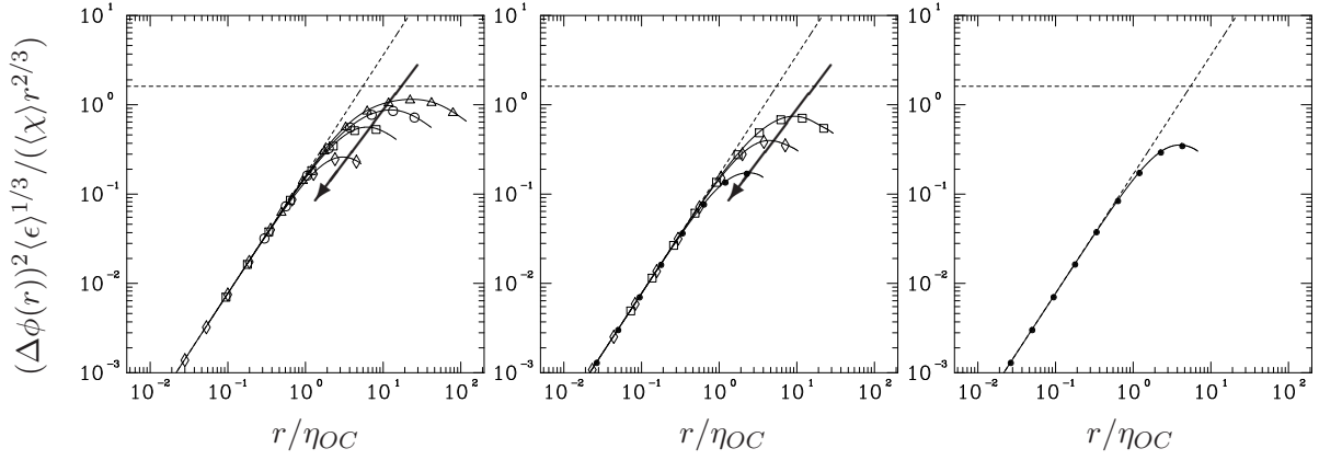
Figure 4.2: Second-order scalar structure function compensated by Obukhov-Corrsin scaling. Frames in the left, middle and right columns are for R_\lambda \sim 140, 240 and 390 respectively. Each choice of symbol on the curves denote a different value of Sc : 1/8 ( \Delta ), 1/32 ( \circ ), 1/128 ( \square ), 1/512 ( \diamond ) and 1/2048 ( \bullet ). Arrows point in the direction of decreasing Schmidt number in each frame. Dashed lines indicate slope 4/3 at small scales (Eq. 4.5) and value of the Obukhov-Corrsin constant C_2 \approx 1.608 (Eq. 4.4).
