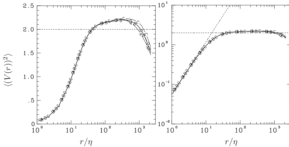
Figure 6.19: Second moment of V along three different Cartesian directions X, Y and Z (lines A, B and C) along with the component averaged plot (line D), for 4096^3 , R_\lambda \sim 650 . (a) (left) log-linear scales to check inertial range behavior (b) (right) log-log scales to check small- r behavior. Dashed lines (positive slope) corresponds to r^{4/3} to check small- r slope. Dashed line (zero slope) at 2.0 for comparison with corresponding K41 result.
