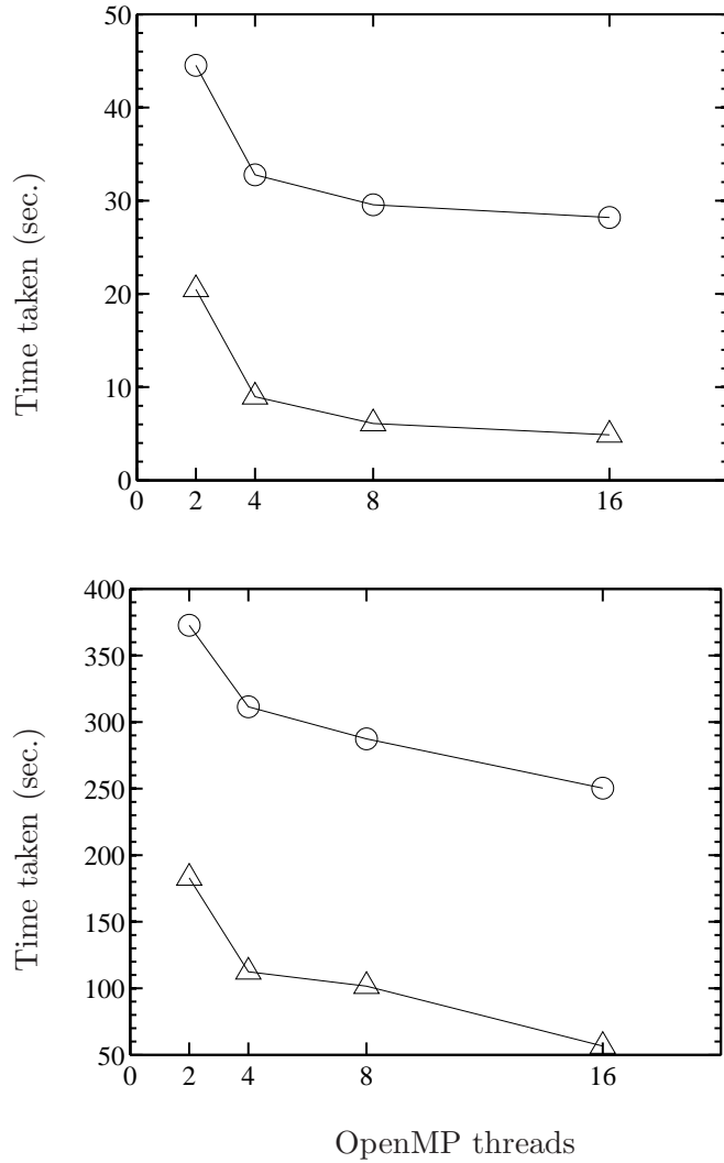
Figure 5.11: Scaling of the angle-averaging code with respect to number of OpenMP threads on Stampede (TACC) for (a) (top) 1024^3 using 2048 cores, (b) (bottom) 2048^3 using 4096 cores. Symbols ( \Delta ) and ( \circ ) correspond to the communication and total times respectively. The difference between the ordinates of the two curves in each frame gives the computation time which is roughly a constant.
