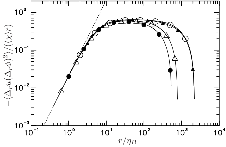
Figure 4.10: Test of Yaglom's relation based on the (component-averaged) mixed velocity-scalar third-order structure function, versus separation scaled by the Batchelor scale. Reynolds and Schmidt number combinations shown are: (i) R_\lambda \approx 650 and Sc = 1/8 ( \Delta ), (ii) R_\lambda \approx 650 and Sc = 1 ( \circ ), (iii) R_\lambda \approx 140 and Sc = 4 ( \bullet ), (iv) R_\lambda \approx 140 and Sc = 64 ( \blacktriangle ). The dashed horizontal line is at height 2/3 . The dotted line of slope 2 shows the small r limit assuming \tilde{S}_{u\phi} = -0.5 (see Table 4.6), which holds approximately for Sc = O(1) or higher.
