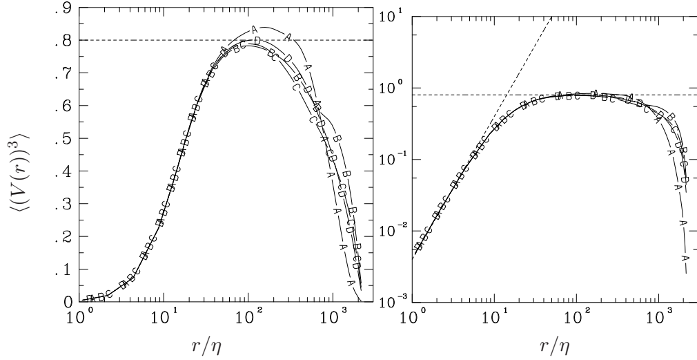
Figure 6.20: Third moment of V along three different Cartesian directions X, Y and Z (lines A, B and C ) along with the component averaged plot (line D ), for 4096^3 , R_\lambda \sim 650 . (a) (left) log-linear scales to check inertial range behavior (b) (right) log-log scales to check small- r behavior. Dashed lines (positive slope) to check the small- r slope (see Eq. 6.25) while dashed line (zero slope) at 0.8 shows the K41 plateau.
