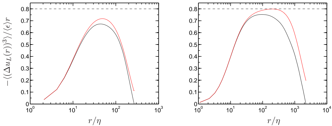
Figure 5.13: Angle-averaged third-order velocity structure function (red), component averaged third-order velocity structure function (black) for (a) (left) 256^3 , R_\lambda \sim 140 , (b) (right) 4096^3 , R_\lambda \sim 650 . Horizontal line at 4/5 shows the asymptotic K41 constant (Eq. 5.1). The structure functions have been averaged in time using seven instantaneous snapshots.
