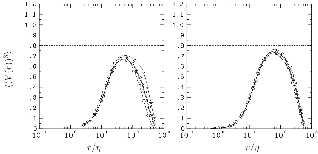
Figure 6.13: Third moment of V along three different Cartesian directions X, Y and Z (lines A, B and C) along with the component averaged plot (line D) at R_\lambda \sim 240 for (a) (left) k_{max}\eta = 1.4 , (b) k_{max}\eta = 5.7 . Dashed lines (positive slope) to check the small- r slope (see Eq. 6.25) while dashed line (zero slope) at 0.8 shows the K41 plateau.
